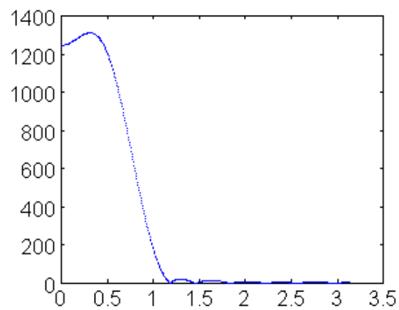
Figure 2.103 Middle filter response
