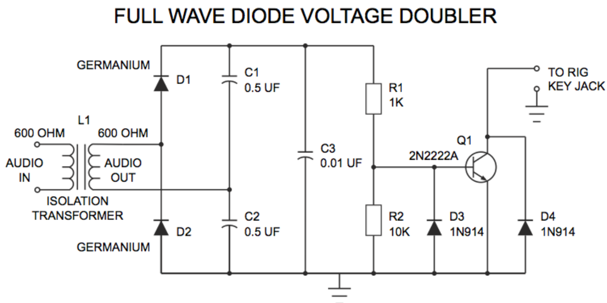
Figure 6.2 CW Keying Circuit
