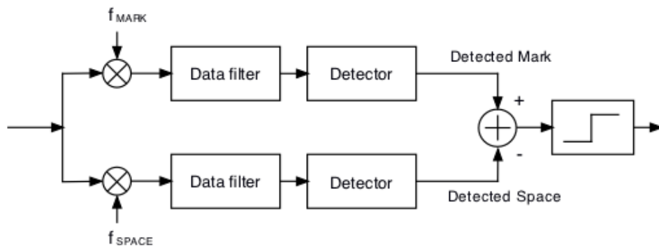
Figure 5.73 Demodulator
